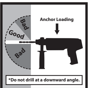
PROPER DRILLING
